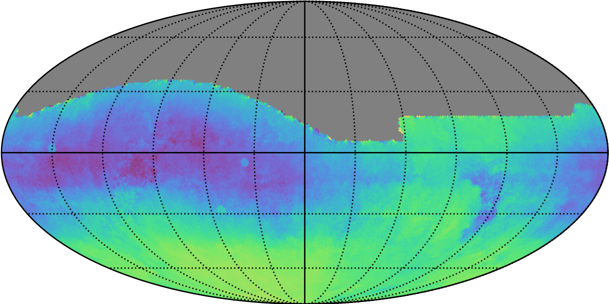
early_ss_template_fpextra2.0_v3.4_10yrs All sky: Parallax-DCR degeneracy @ 24.0
