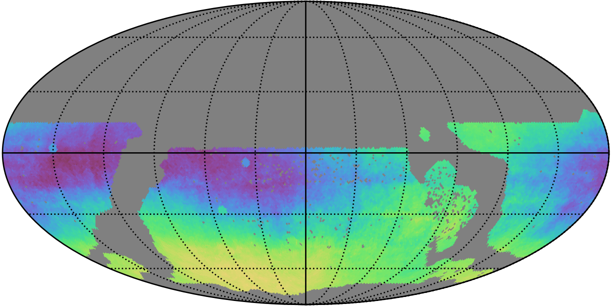
early_ss_template_fpextra2.0_v3.4_10yrs WFD: Parallax-DCR degeneracy @ 22.4
