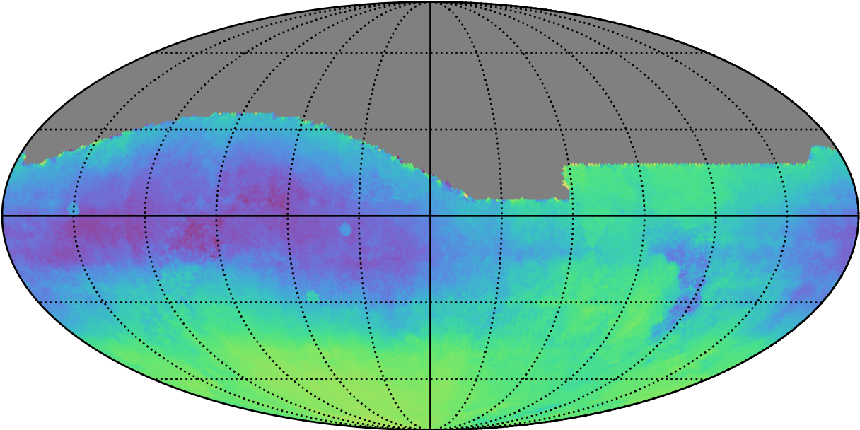
early_ss_template_fpextra2.0_v3.4_10yrs All sky: Parallax-DCR degeneracy @ 22.4
