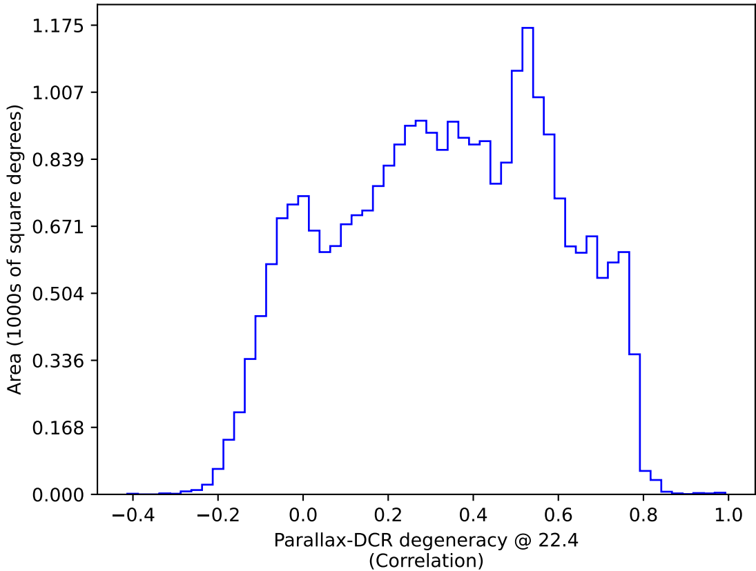
early_ss_template_fpextra2.0_v3.4_10yrs All sky: Parallax-DCR degeneracy @ 22.4
