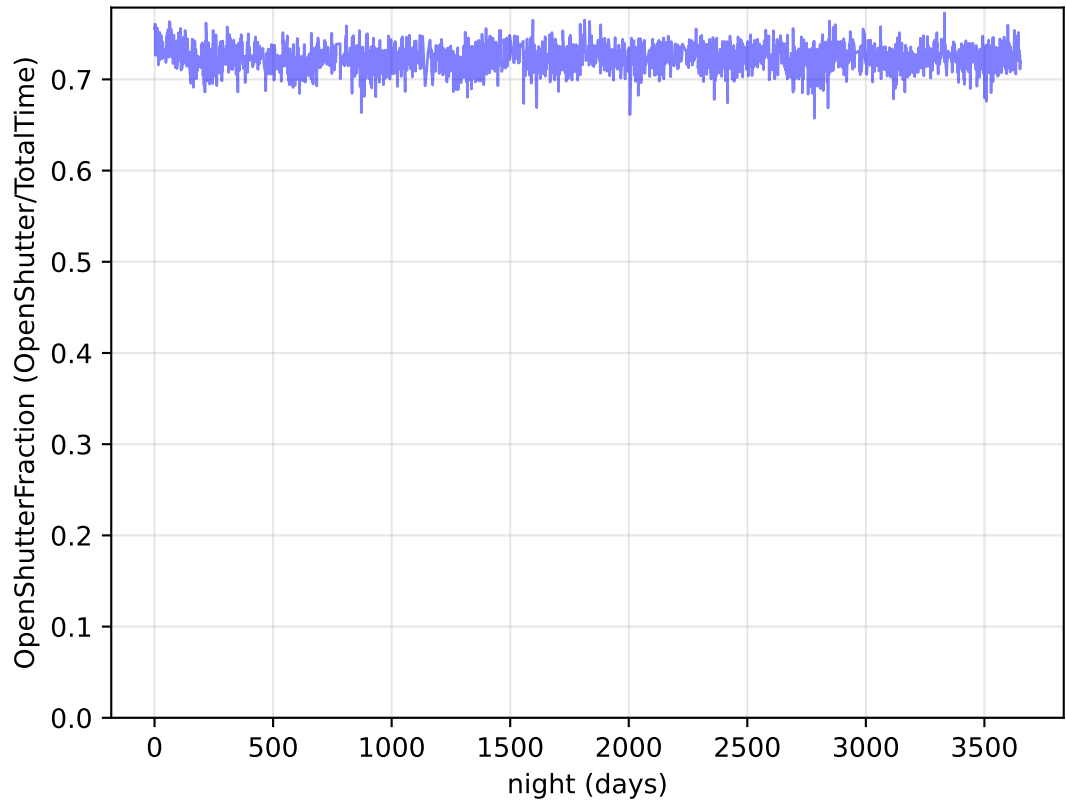
early_ss_template_fpextra2.0_v3.4_10yrs Per night: OpenShutterFraction
