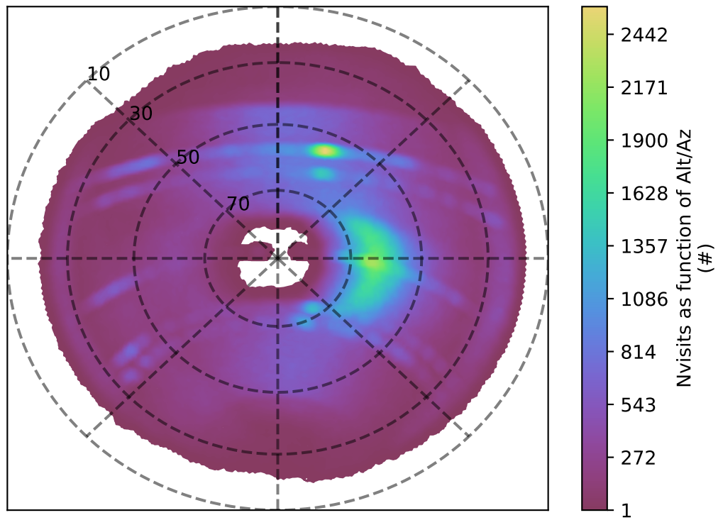
early_ss_template_fpextra2.0_v3.4_10yrs z band: Nvisits as function of Alt/Az
