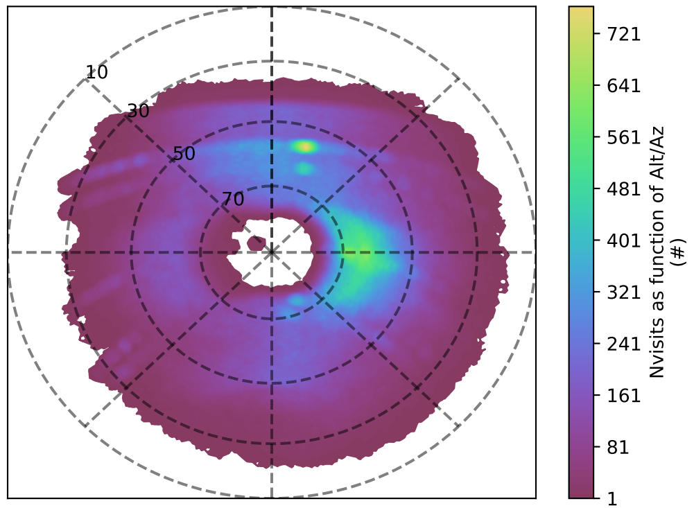
early_ss_template_fpextra2.0_v3.4_10yrs u band: Nvisits as function of Alt/Az
