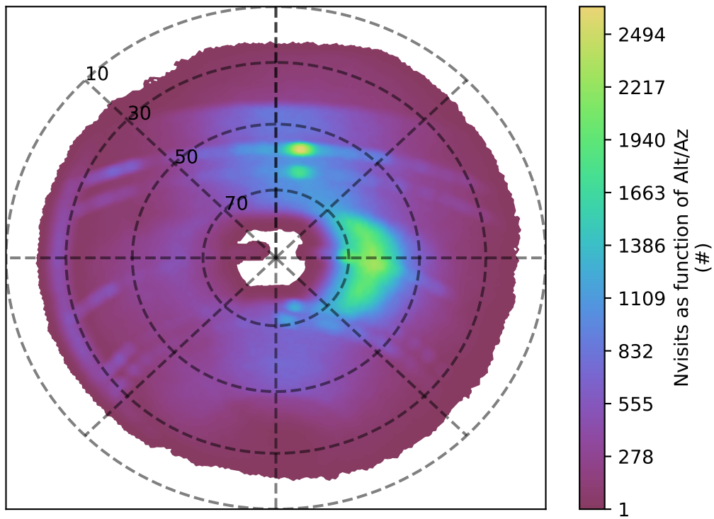
early_ss_template_fpextra2.0_v3.4_10yrs r band: Nvisits as function of Alt/Az
