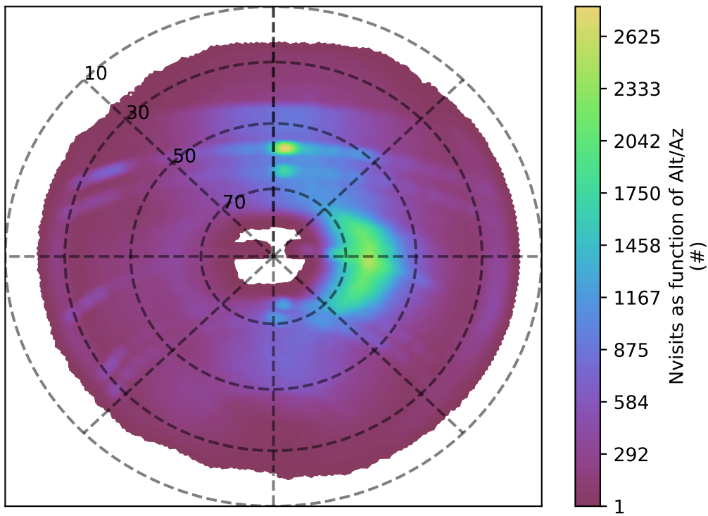
early_ss_template_fpextra2.0_v3.4_10yrs i band: Nvisits as function of Alt/Az
