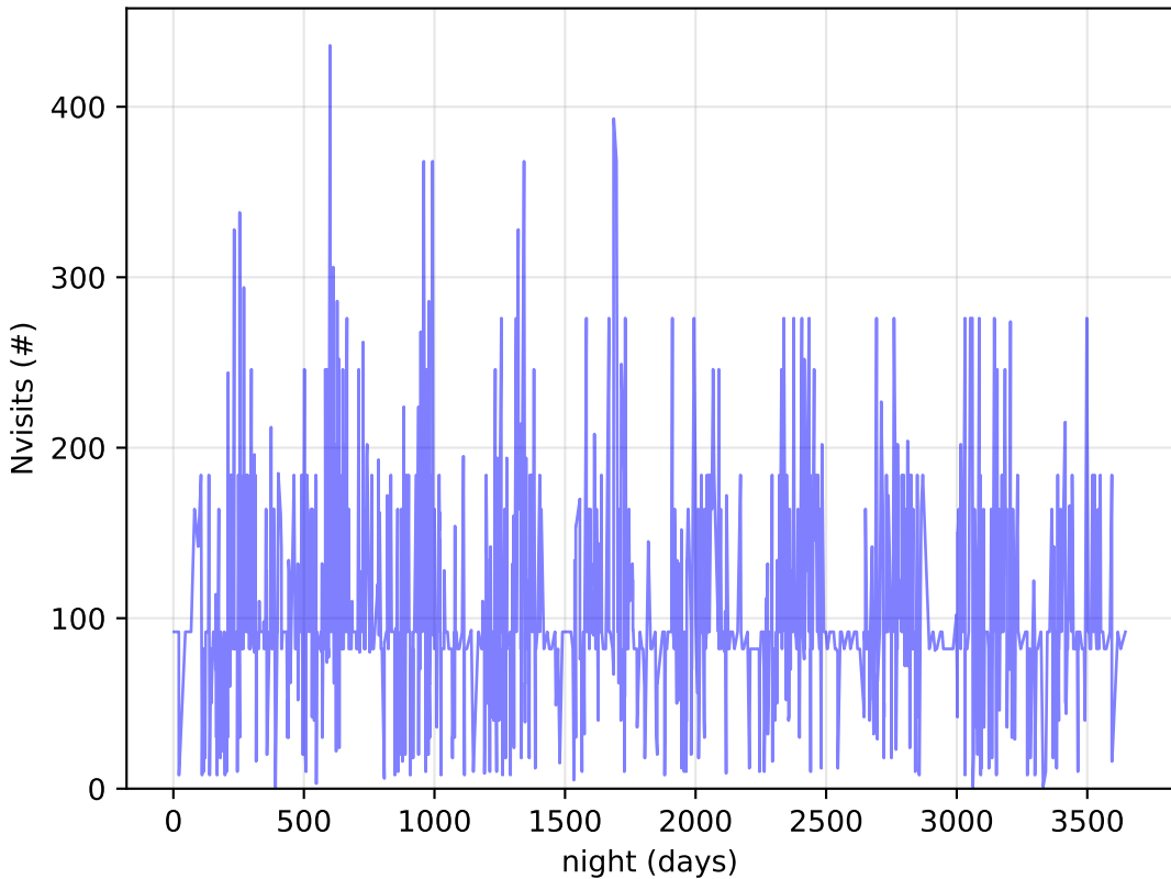
early_ss_template_fpextra2.0_v3.4_10yrs DDF: Nvisits
