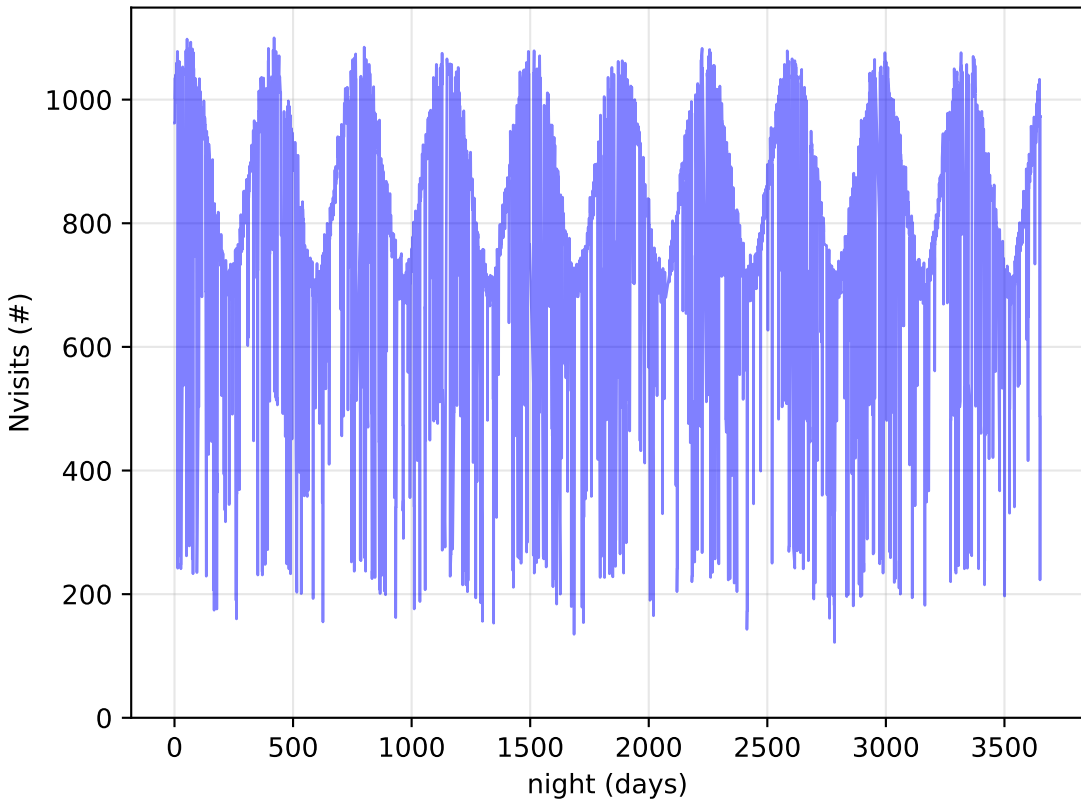
early_ss_template_fpextra2.0_v3.4_10yrs All visits: Nvisits
