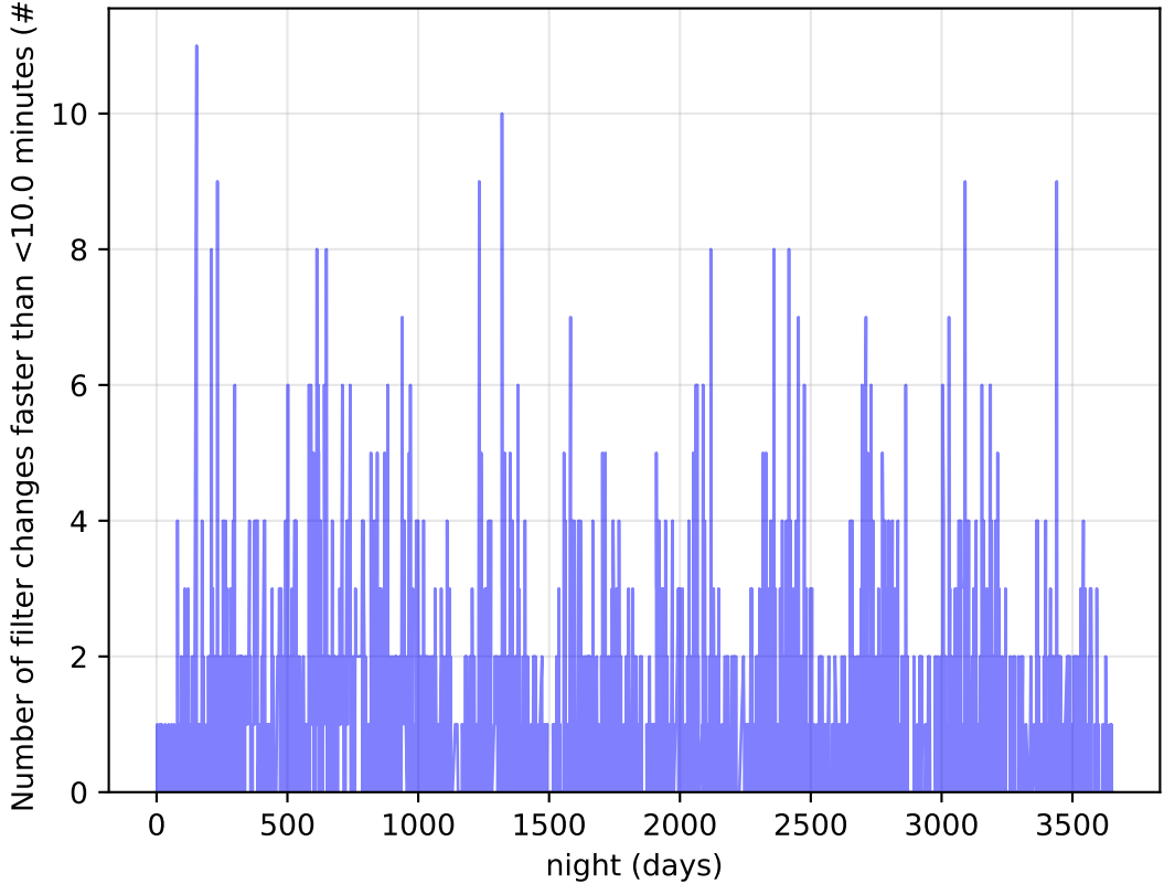
early_ss_template_fpextra2.0_v3.4_10yrs Per Night: Number of filter changes faster than <10.0 minutes
