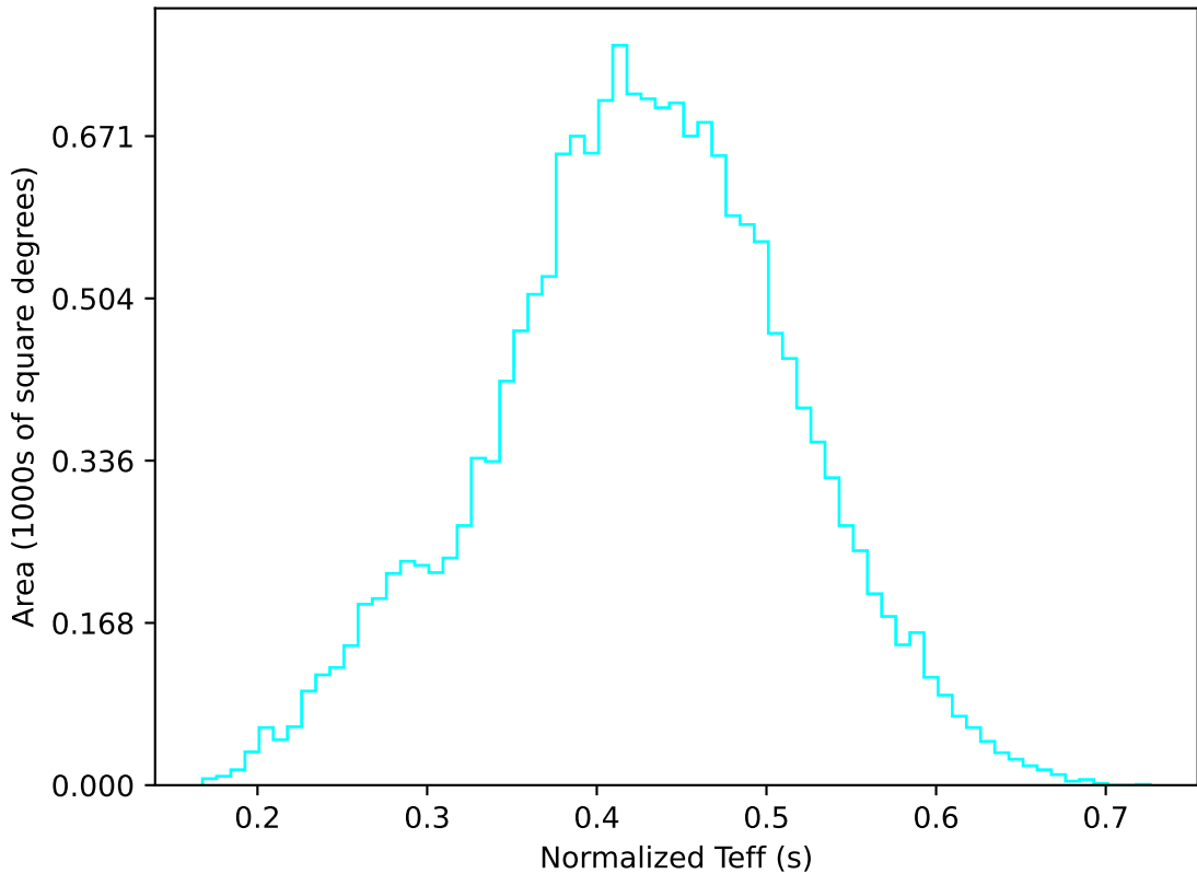
early_ss_template_fpextra2.0_v3.4_10yrs WFD u band: Normalized Teff
