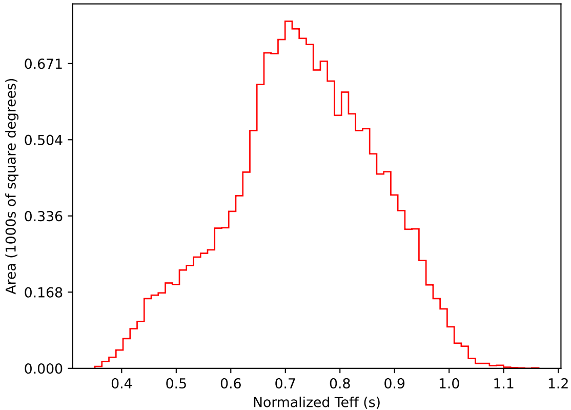
early_ss_template_fpextra2.0_v3.4_10yrs WFD i band: Normalized Teff
