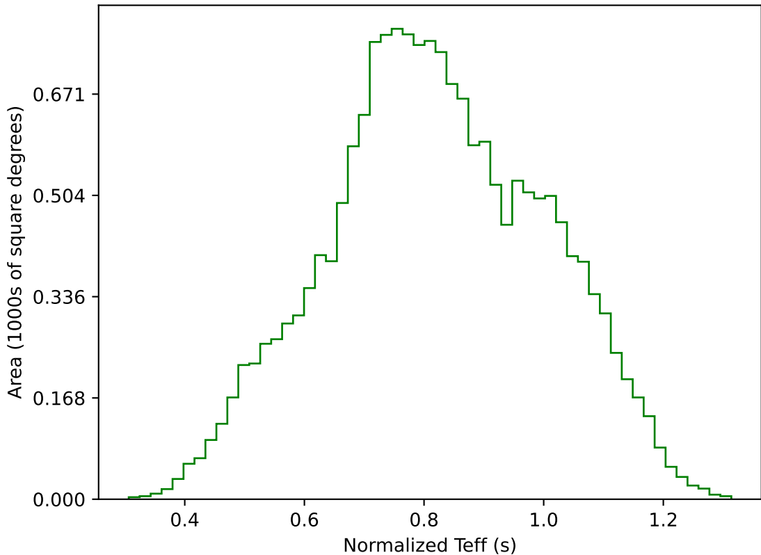
early_ss_template_fpextra2.0_v3.4_10yrs WFD g band: Normalized Teff
