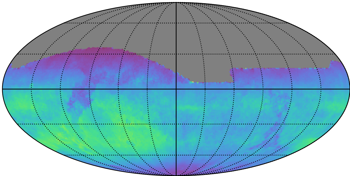
early_ss_template_fpextra2.0_v3.4_10yrs All sky z band: Normalized Teff
