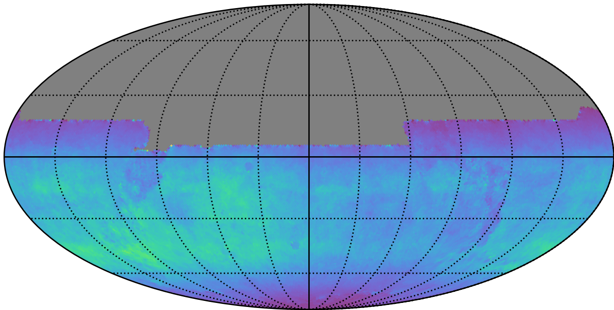
early_ss_template_fpextra2.0_v3.4_10yrs All sky y band: Normalized Teff
