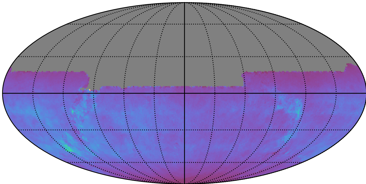
early_ss_template_fpextra2.0_v3.4_10yrs All sky u band: Normalized Teff
