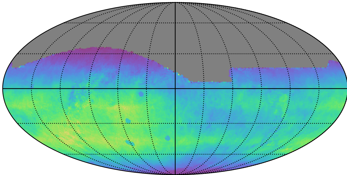
early_ss_template_fpextra2.0_v3.4_10yrs All sky r band: Normalized Teff
