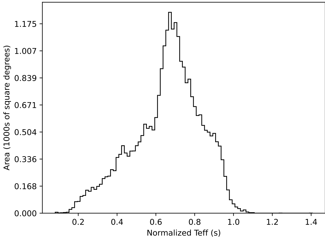
early_ss_template_fpextra2.0_v3.4_10yrs All sky all bands: Normalized Teff
