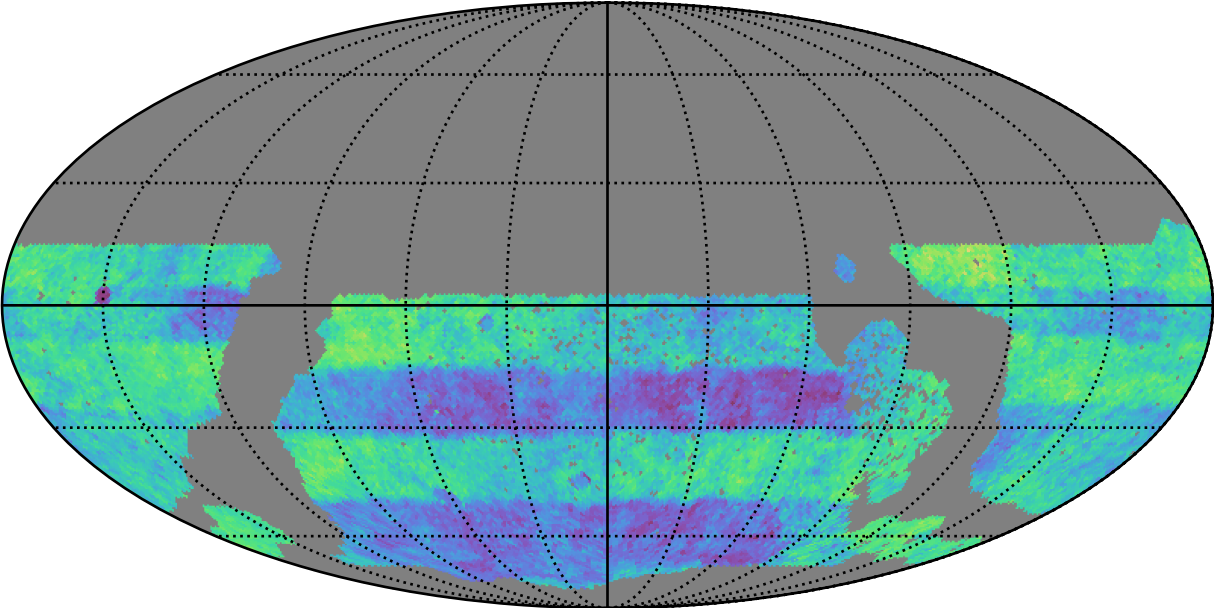
early_ss_template_fpextra2.0_v3.4_10yrs WFD: Normalized Proper Motion Uncert @ 24.0
