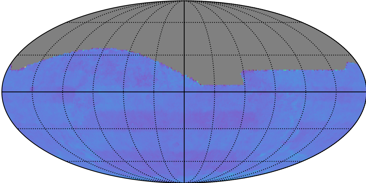
early_ss_template_fpextra2.0_v3.4_10yrs All sky: Normalized Proper Motion Uncert @ 24.0
