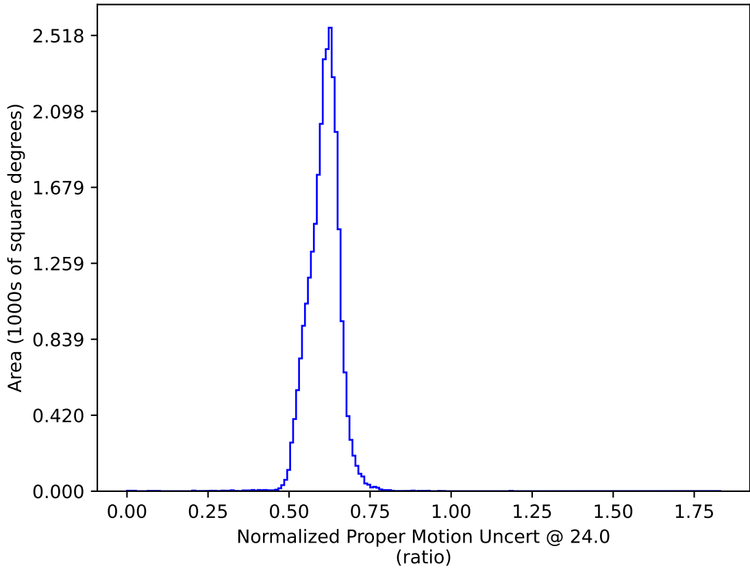
early_ss_template_fpextra2.0_v3.4_10yrs All sky: Normalized Proper Motion Uncert @ 24.0
