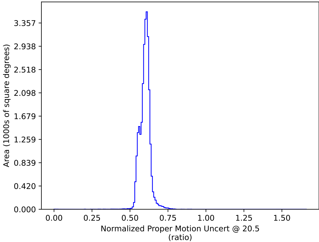
early_ss_template_fpextra2.0_v3.4_10yrs All sky: Normalized Proper Motion Uncert @ 20.5
