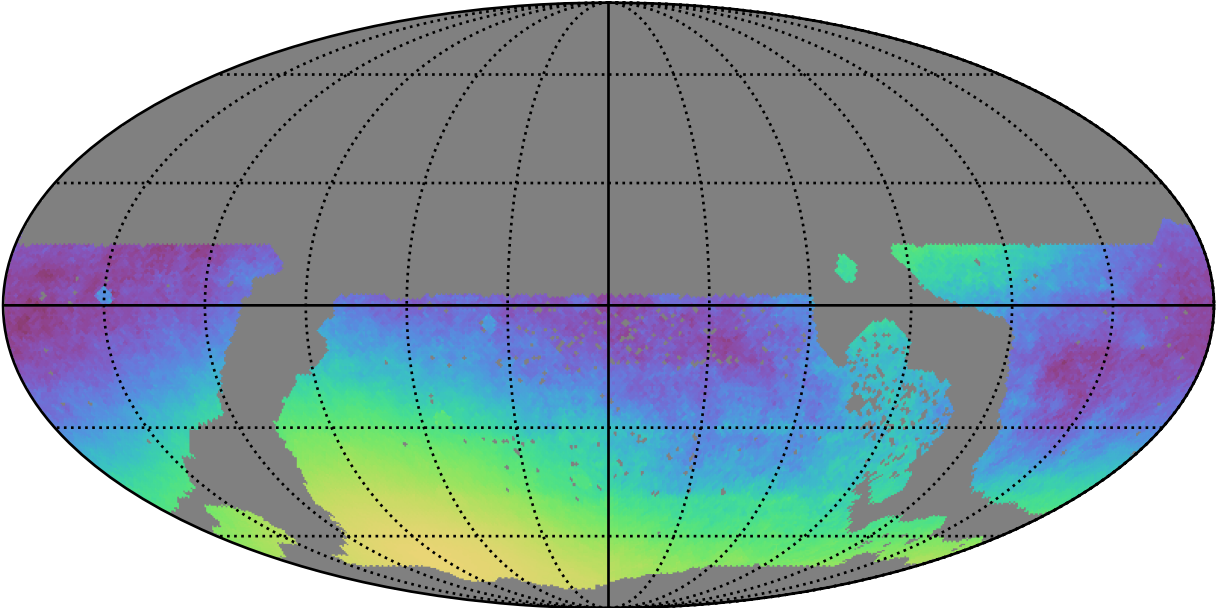
early_ss_template_fpextra2.0_v3.4_10yrs WFD: Normalized Parallax Uncert @ 24.0
