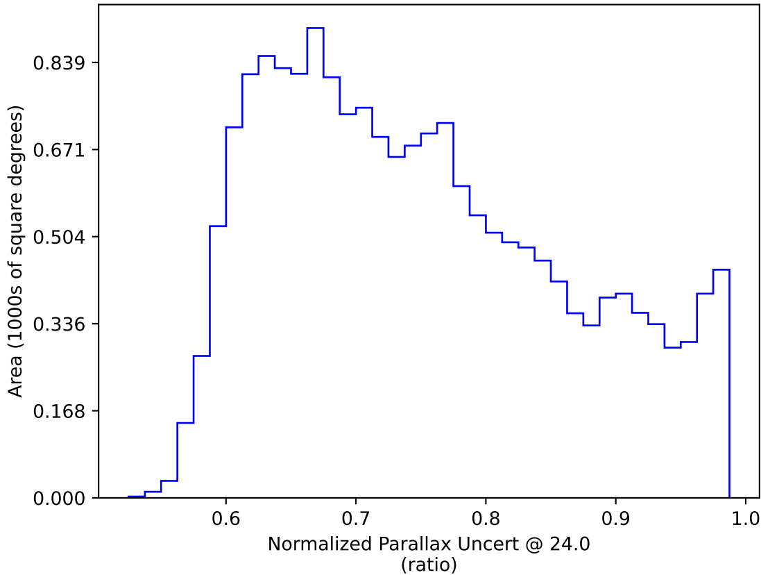
early_ss_template_fpextra2.0_v3.4_10yrs WFD: Normalized Parallax Uncert @ 24.0
