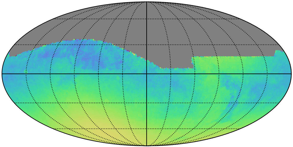
early_ss_template_fpextra2.0_v3.4_10yrs All sky: Normalized Parallax Uncert @ 24.0
