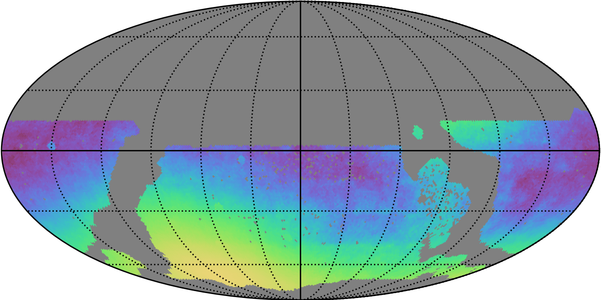
early_ss_template_fpextra2.0_v3.4_10yrs WFD: Normalized Parallax Uncert @ 22.4
