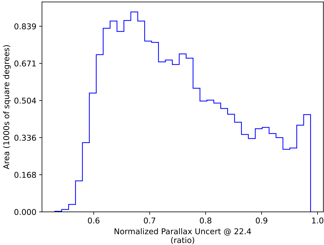
early_ss_template_fpextra2.0_v3.4_10yrs WFD: Normalized Parallax Uncert @ 22.4
