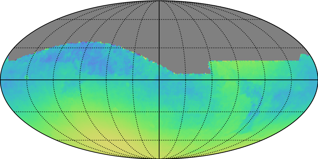
early_ss_template_fpextra2.0_v3.4_10yrs All sky: Normalized Parallax Uncert @ 22.4
