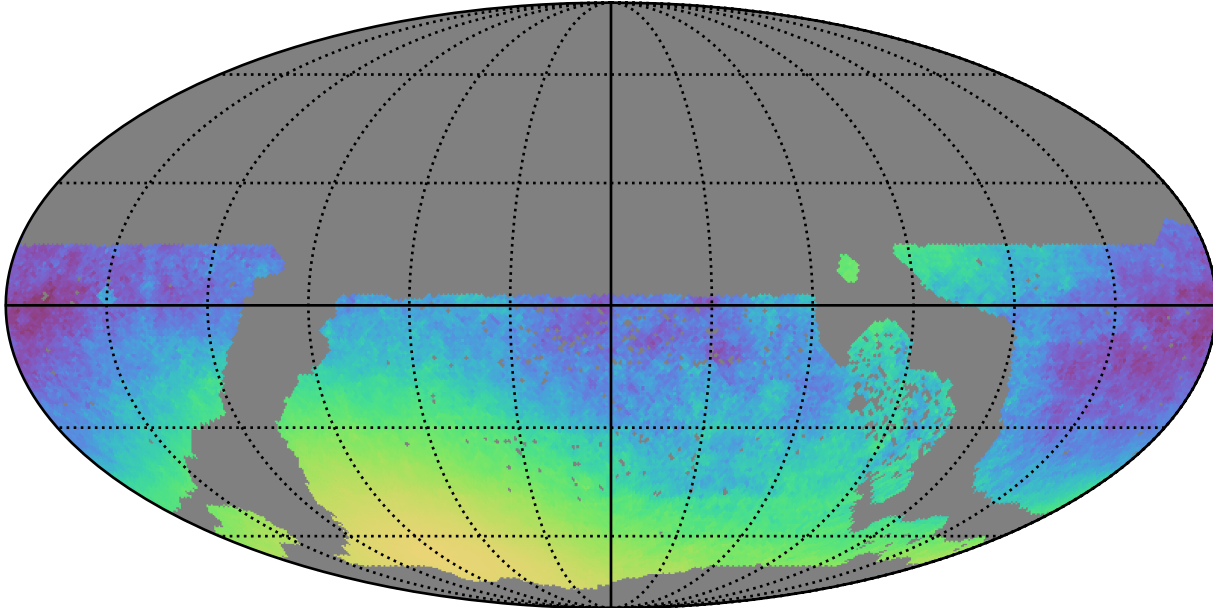
early_ss_template_fpextra2.0_v3.4_10yrs WFD y band only: Normalized Parallax Uncert @ 21.3
