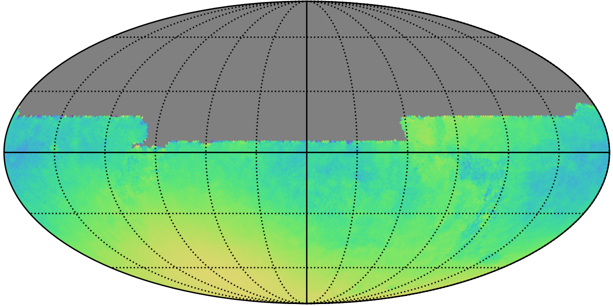
early_ss_template_fpextra2.0_v3.4_10yrs All sky y band only: Normalized Parallax Uncert @ 21.3
