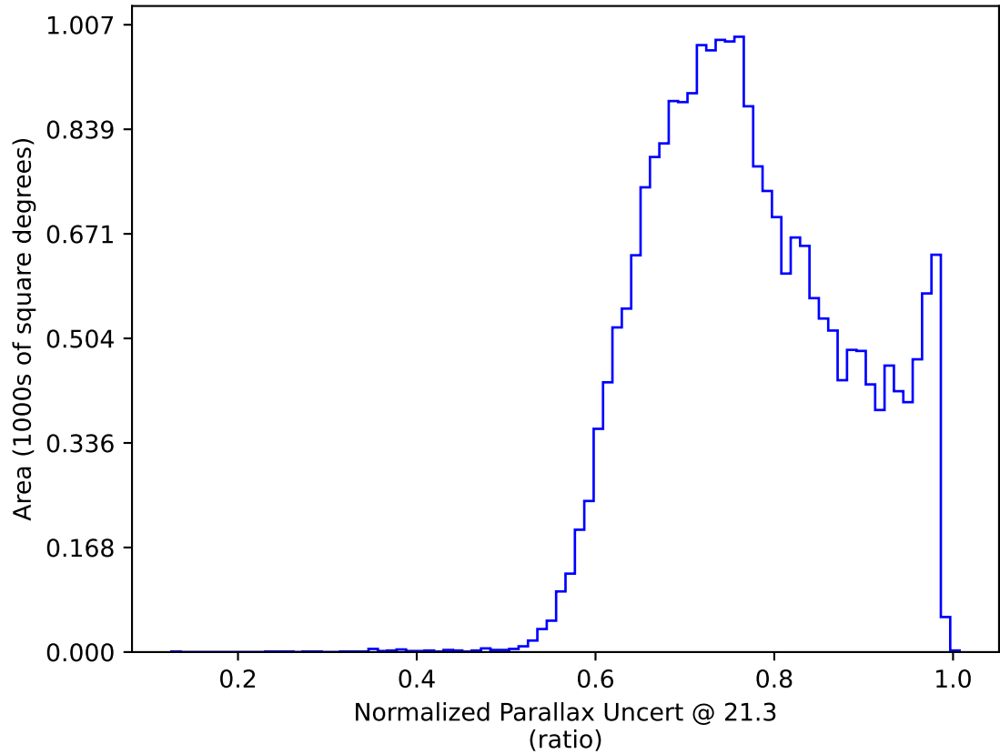
early_ss_template_fpextra2.0_v3.4_10yrs All sky y band only: Normalized Parallax Uncert @ 21.3
