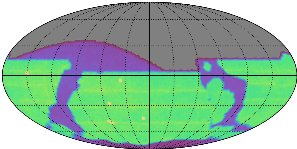
early_ss_template_fpextra2.0_v3.4_10yrs All sky all bands: N Unique Nights
