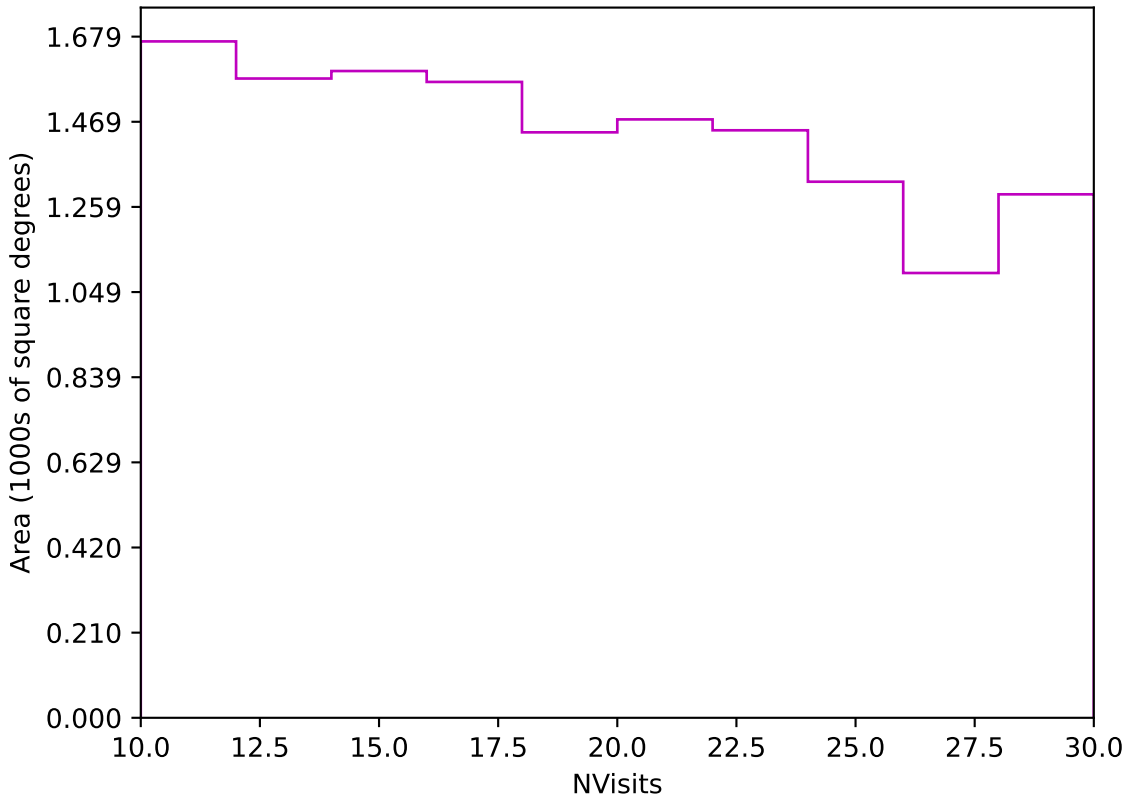
early_ss_template_fpextra2.0_v3.4_10yrs Yr 3-4 z band: NVisits
