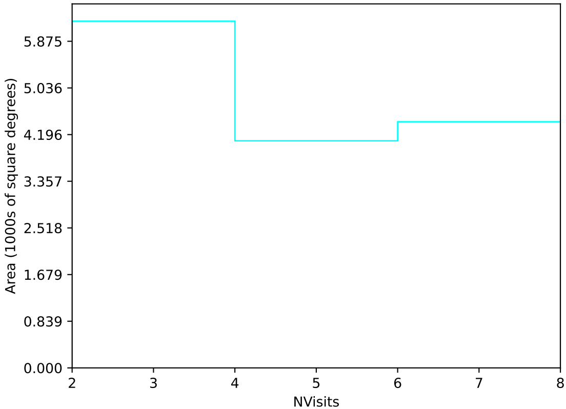
early_ss_template_fpextra2.0_v3.4_10yrs Yr 3-4 u band: NVisits
