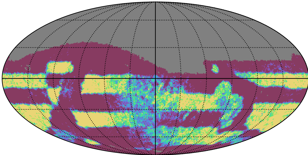
early_ss_template_fpextra2.0_v3.4_10yrs Yr 3-4 r band: NVisits
