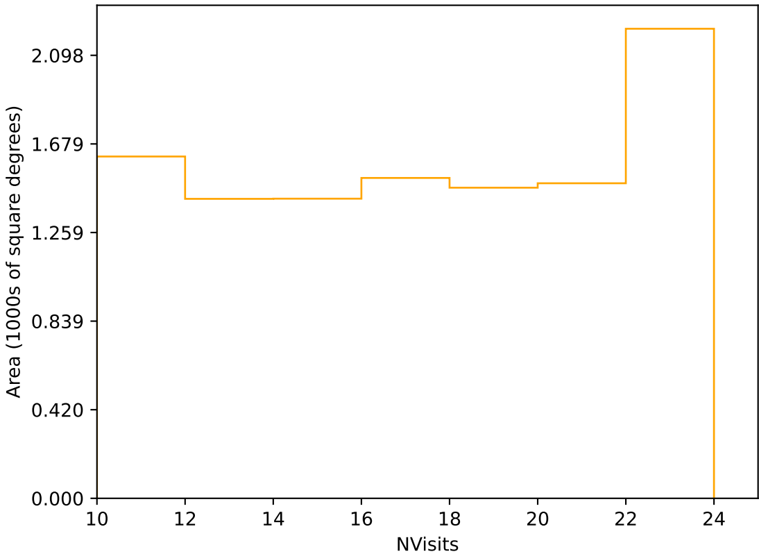
early_ss_template_fpextra2.0_v3.4_10yrs Yr 3-4 r band: NVisits
