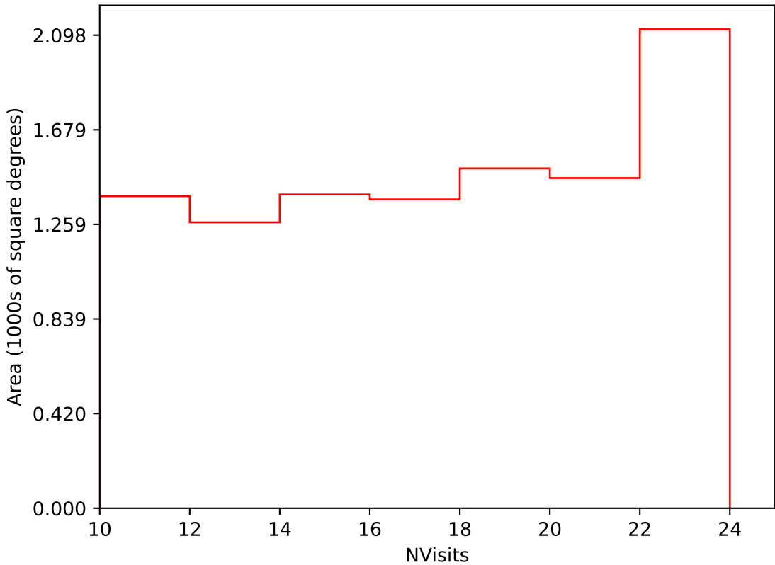
early_ss_template_fpextra2.0_v3.4_10yrs Yr 3-4 i band: NVisits
