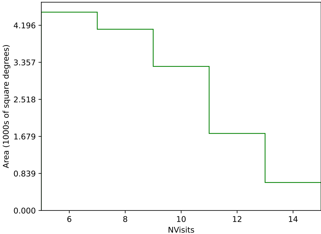
early_ss_template_fpextra2.0_v3.4_10yrs Yr 3-4 g band: NVisits
