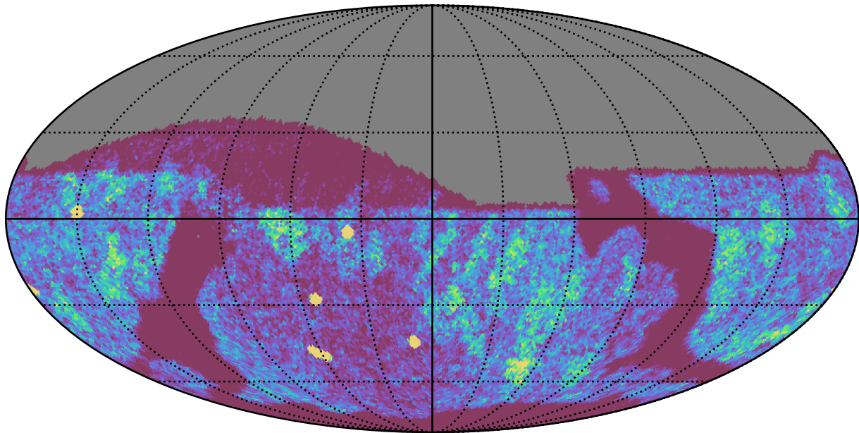
early_ss_template_fpextra2.0_v3.4_10yrs Yr 1 z band: NVisits
