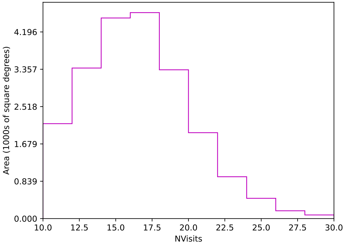
early_ss_template_fpextra2.0_v3.4_10yrs Yr 1 z band: NVisits
