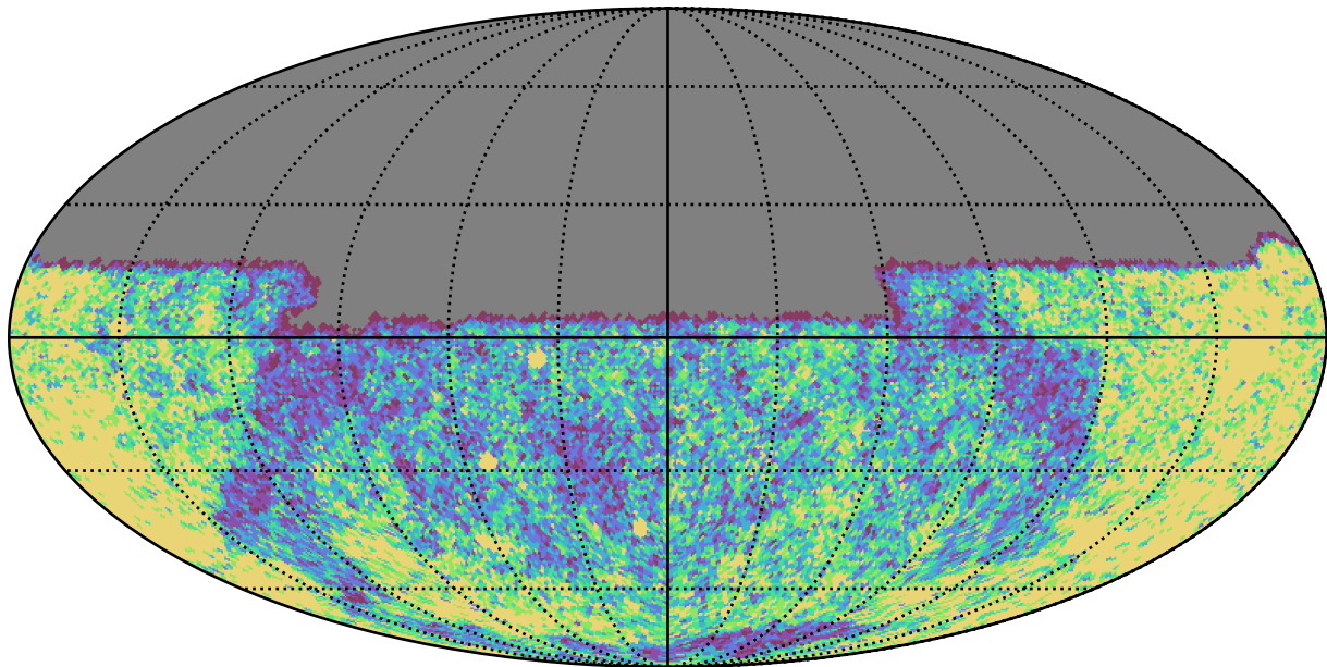
early_ss_template_fpextra2.0_v3.4_10yrs Yr 1 u band: NVisits
