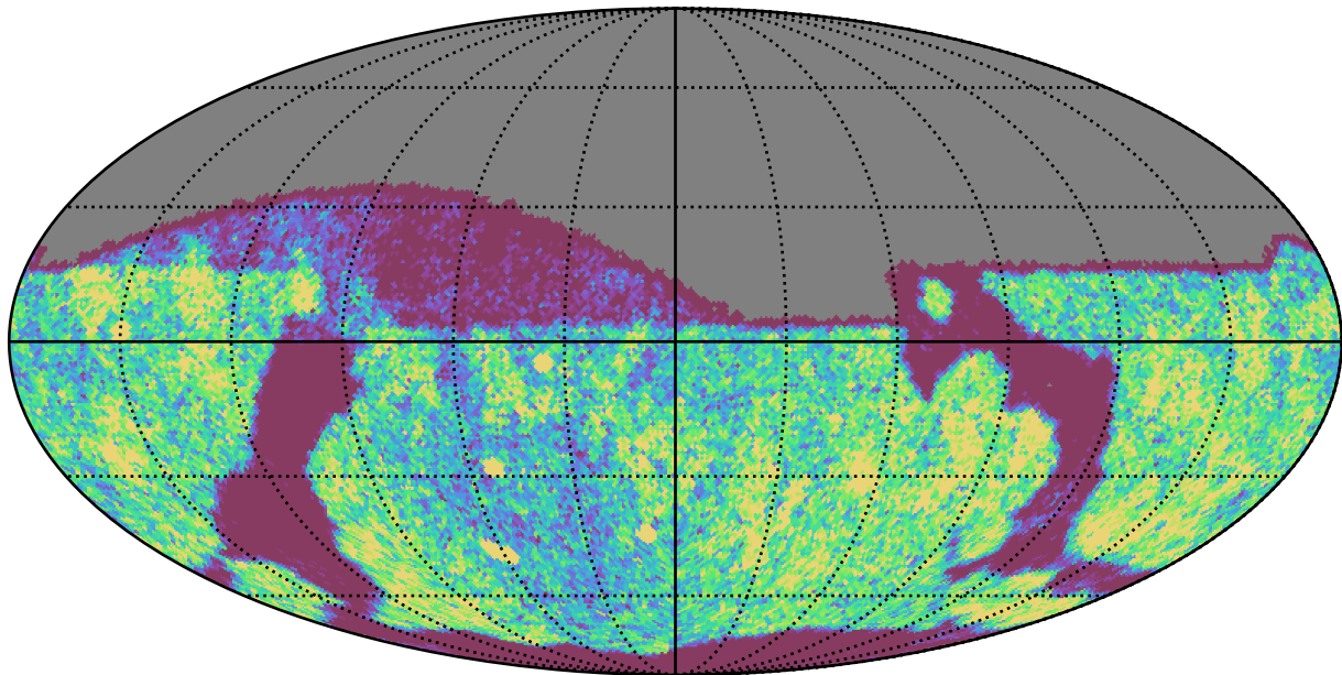
early_ss_template_fpextra2.0_v3.4_10yrs Yr 1 i band: NVisits
