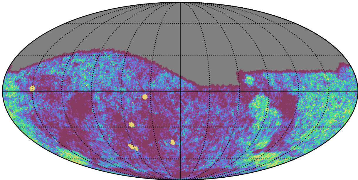
early_ss_template_fpextra2.0_v3.4_10yrs Yr 1 g band: NVisits
