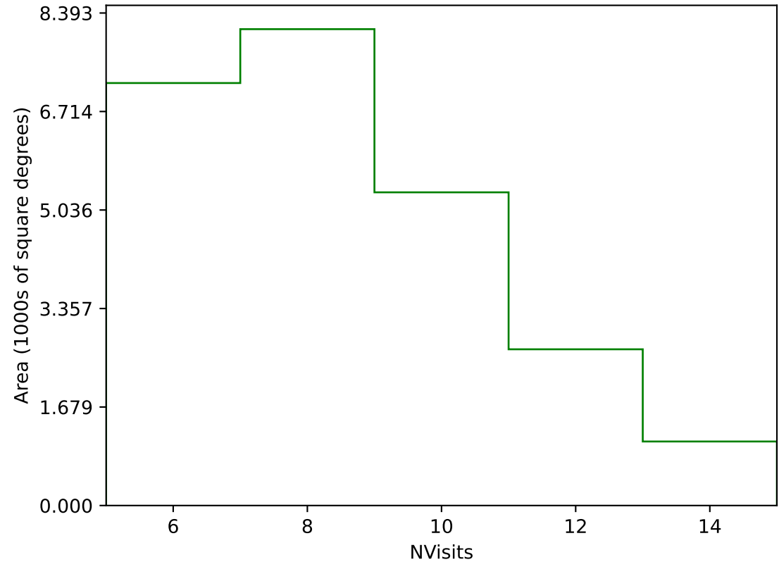
early_ss_template_fpextra2.0_v3.4_10yrs Yr 1 g band: NVisits
