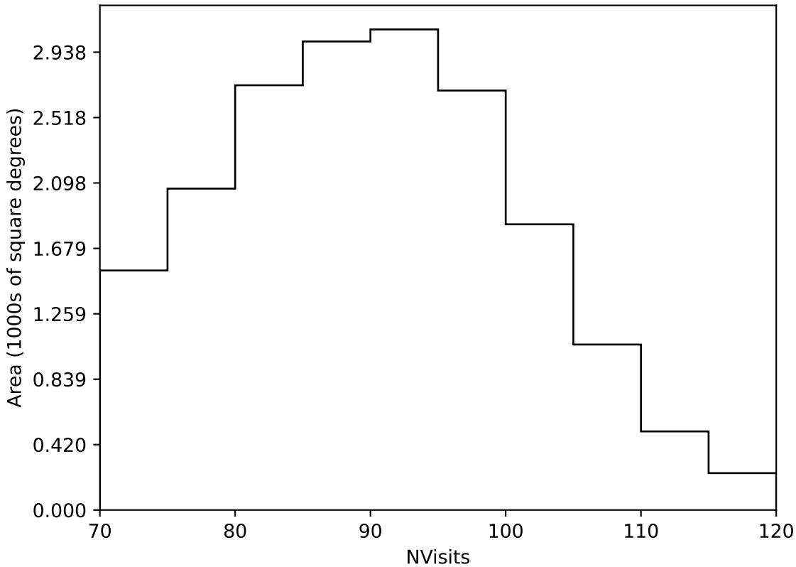
early_ss_template_fpextra2.0_v3.4_10yrs Yr 1 all bands: NVisits
