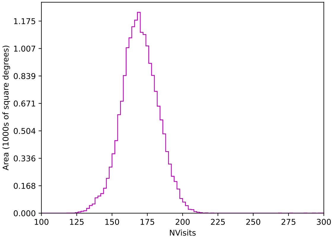
early_ss_template_fpextra2.0_v3.4_10yrs WFD z band: NVisits
