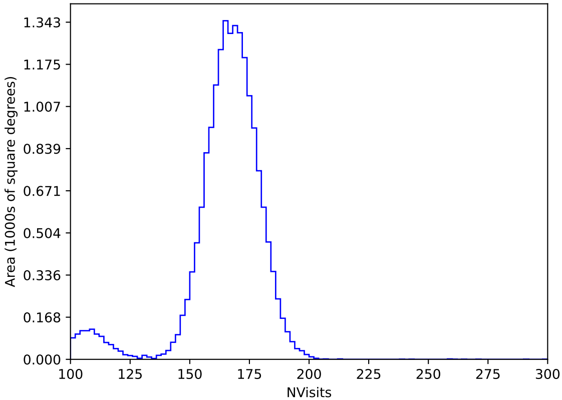
early_ss_template_fpextra2.0_v3.4_10yrs WFD y band: NVisits
