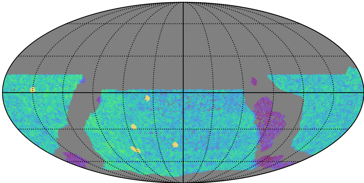
early_ss_template_fpextra2.0_v3.4_10yrs WFD u band: NVisits
